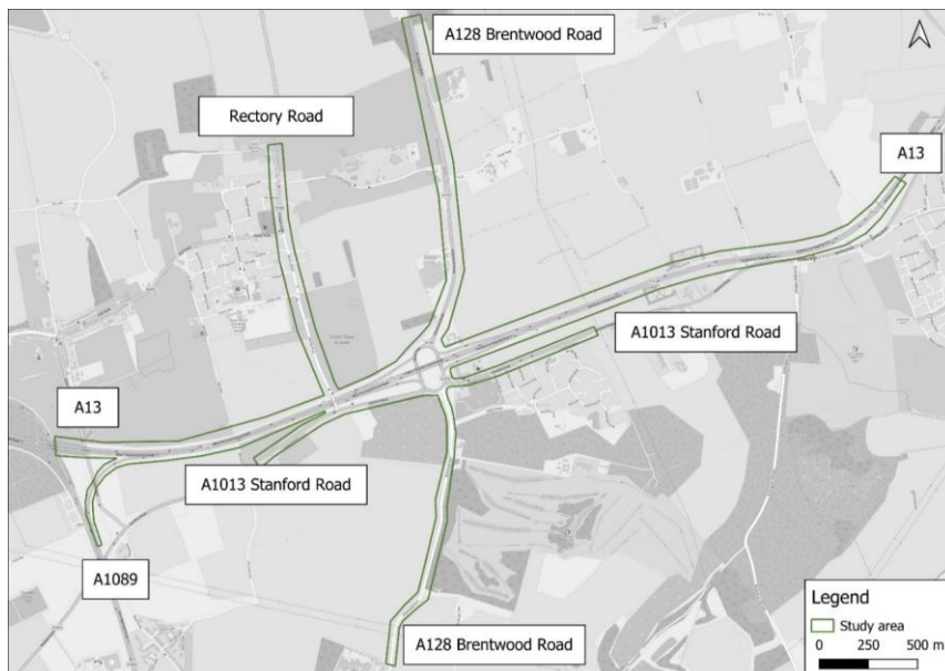
Plate N.2 Orsett Cock junction VISSIM model extents
