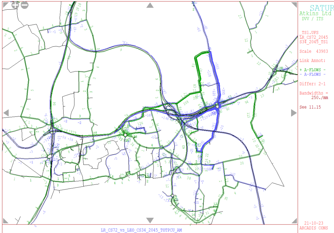
Plate N.9 2045 AM plots VISSIM delays hard coded into SATURN, Thurrock
